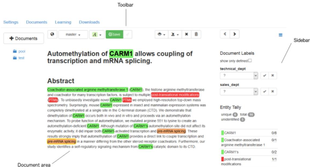
tagtog annotation editor with text span annotations and document labels. The editor is mainly divided into: Document area, Toolbar and Sidebar.
